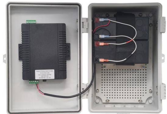
10A Solar, 30W PoE Controller Inside
