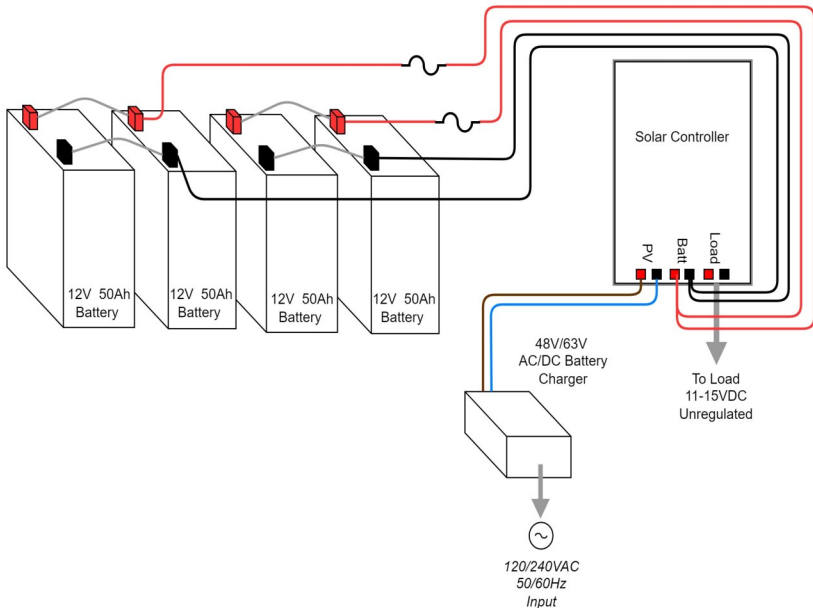
UPS-STL-500/600 12V 4 Battery Configuration
