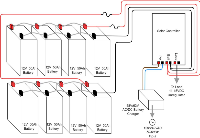
UPS-STL-500/600 12V 8 Battery Configuration
