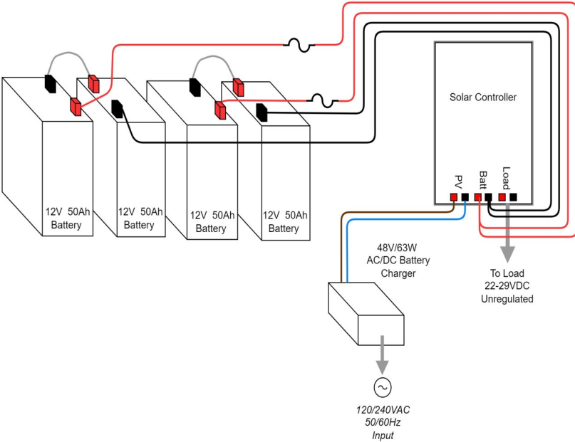
UPS-STL-500/600 24V 4 Battery Configuration
