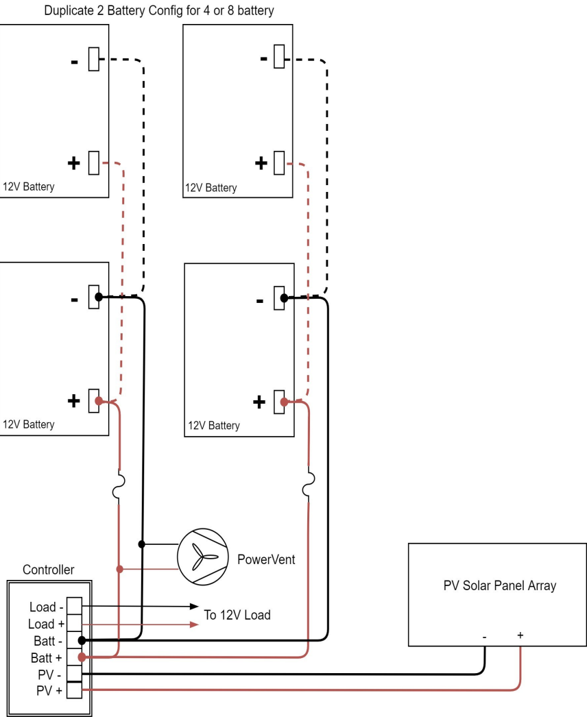
RemotePro 12V Wiring Diagram
