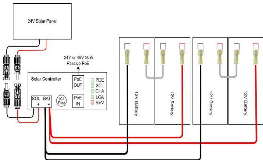
24V Battery Configuration
